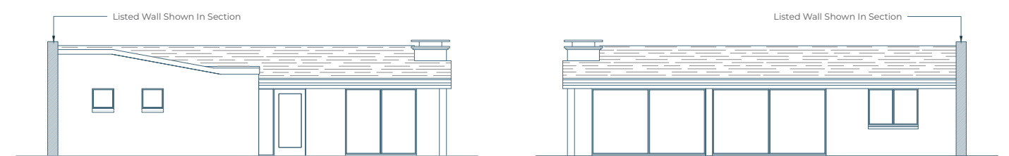
Plot 2 - West Elevation
